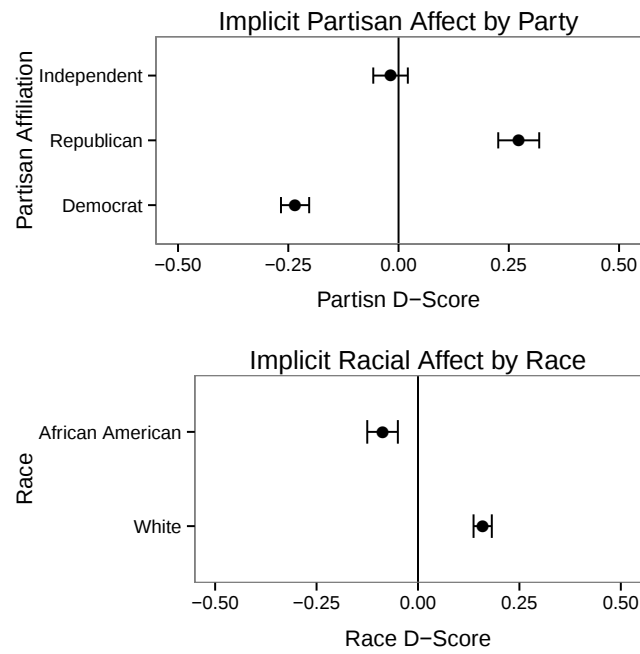
Figure 4: Distribution of D-scores for the Partisan and African American/European American BIATs
